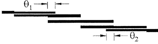
Fig. 2. Layout for a third-order filter. Over-couplings are applied to the end stages.
