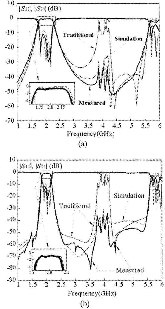
Fig. 3. Simulated and measured responses for Chebyshev bandpass filters. The center frequency f_o = 2 GHz and passband ripple = 0.1 dB. The substrate has \epsilon_r = 10.2 and thickness h = 1.27 mm. (a) Responses of a third-order filter with fractional bandwidth \Delta = 20\% . The electrical lengths for over-coupling at the end stages are \theta_1 = 12.7^\circ and \theta_2 = 17.2^\circ . (b) Responses of a fifth-order filter with \Delta = 15\% , \theta_1 = 15.1^\circ and \theta_2 = 18.8^\circ .
